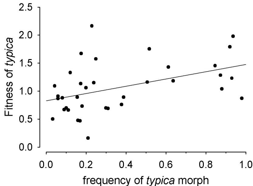
Figure 3. Relative fitness of adult typica (normal, pale form) compared with carbonaria (melanic form) in 35 field experiments with the peppered moth, Biston betularia . The survival data are plotted against the frequency of typica in the population, and the trend shows that adults of each form tend to have higher survival in areas where its own form is most abundant, as expected under the industrial melanism hypothesis. The equation for the best-fitting line is y = 0.83 + 0.65x ; r^2 = 0.20 , P=0.007 ). The data are from Cook (2000); see also Lees (1981). Laurence Cook has told me he doesn't believe the simple regression analysis performed here is sensible, as different groups of experiments were done in very different ways and with different sample sizes. However, I am merely using this regression as a conservative heuristic tool to display the data, because I believe it shows the results clearly. Cook's own (2000) sample-size-weighted analysis of the data after log-transforming the relative fitness values gave similar results ( P < 0.001 ).
