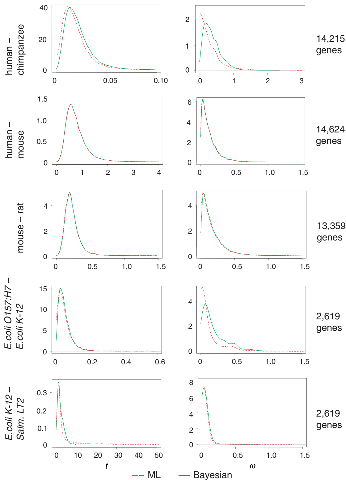
FIG. 4. Distributions (smoothed histograms) of Bayesian and ML estimates of t and \omega from mammalian and bacterial pairwise gene comparisons. Numbers of genes analyzed in each comparison are shown in the right part of the figure.
