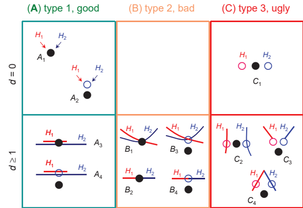
Fig. 2. Classification of Bayesian model-selection problems involving two equally right or equally wrong models, each with d free parameters. Solid circles represent the true model, while the lines represent the parameter space of the compared models, with the empty circles to be the best-fitting parameter value ( \theta^* ). The two models are equally right (with D_1 = D_2 = 0 ) if the solid and empty circles coincide, and equally wrong (with D_1 = D_2 > 0 ) if they are separate. The models are ‘indistinct’ if the two empty circles coincide (as in A and B), and are ‘distinct’ if they are separate (as in C). The green, orange, and red boxes indicate the three different asymptotic behaviors of Bayesian model selection when the data size n \rightarrow \infty .
