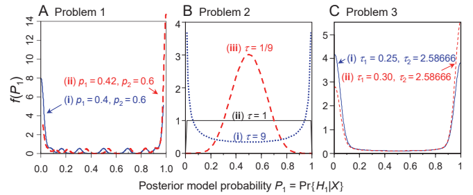
Fig. 3. The distribution of posterior model probability P_1 = \mathbb{P}\{H_1|x\} in three inference problems. (A) Problem 1 (fair-coin paradox) is for a coin-tossing experiment, where the true model is p = 0.5 (a fair coin), and the compared models are (i) H_1 : p = 0.4 and H_2 : p = 0.6 so that the two models are equally wrong; and (ii) H_1 : p = 0.42 and H_2 : p = 0.6 so that H_1 is less wrong than H_2 . The data size (the number of coin tosses) is 10^3 . (B) Problem 2 (fair-balance paradox) is for a normal-distribution example in which the true model is \mathbb{N}(0, 1) , and the two compared models are H_1 : \mathbb{N}(\mu, 1/\tau) , \mu < 0 and H_2 : \mathbb{N}(\mu, 1/\tau) , \mu > 0 , with variance 1/\tau given. The two models are equally right when \tau = 1 and equally wrong but indistinct when \tau = 1/9 or 9 . The data size is n = 10^3 . The plots for n = 100 or \infty are nearly the same. (C) Problem 3 (fair-balance paradox) is for a normal-distribution example in which the true model is \mathbb{N}(0, 1) , and the two compared models are H_1 : \mathbb{N}(\mu, 1/\tau_1) and H_2 : \mathbb{N}(\mu, 1/\tau_2) , with (i) \tau_1 = 0.25 , \tau_2 = 2.586666 , so that the two models are equally wrong and (ii) \tau_1 = 0.30 , \tau_2 = 2.586666 , so that H_1 is less wrong than H_2 . The prior is \mu \sim \mathbb{N}(0, 1/\xi) under each model, with \xi = 1 . The data size is n = 100 . All densities are estimated by simulating 10^5 samples for P_1 .
