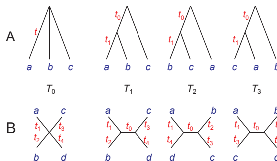
Fig. 1. (A) The three binary rooted trees for three species T_1, T_2, and T_3 and the star tree T_0 . (B) The three binary unrooted trees for four species T_1, T_2, and T_3 and the star tree T_0 . The branch length parameters are shown next to the branches, measured by the expected number of nucleotide changes per site. In the star-tree simulations, the star tree is used to generate data, which are analyzed to calculate the posterior probabilities for the three binary trees, with the star tree excluded.
