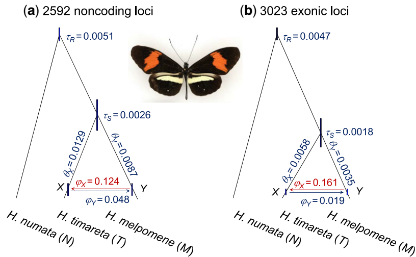
FIG. 2. Species tree or BDI model for Heliconius melpomene , H. timareta , and H. numata . The branches are drawn to represent the posterior means of divergence/introgression times obtained from BPP analysis of (a) the 2,592 noncoding and (b) the 3,023 exonic loci from chromosome 1, while the node bars represent the 95% HPD CIs. See table 1 for estimates of all parameters. Photo of H. timareta courtesy of James Mallet.
