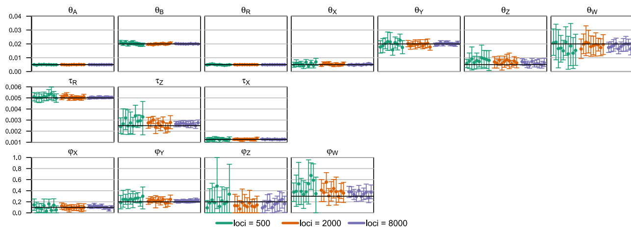
FIG. 8. Posterior means and the 95% HPD CIs in 10 replicate datasets of L = 500, 2,000 , and 8,000 loci, simulated and analyzed under the double-BDI model of figure 6a. The MCMC samples are postprocessed using the \beta - \gamma algorithm before they are summarized (e.g. fig. 7). Eight parameters are involved in the label-switching unidentifiability: \varphi_X, \varphi_Y, \theta_X, \theta_Y, \varphi_Z, \varphi_W, \theta_Z , and \theta_W (see fig. 6).
