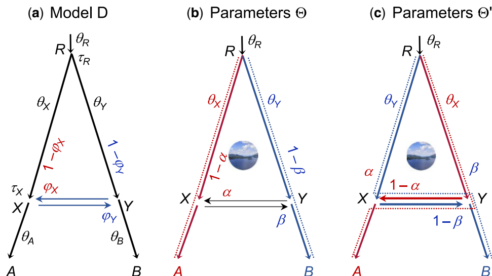
FIG. 1. (a) Species tree or MSci model for two species (A and B) with a bidirectional introgression at time \tau_X = \tau_Y , identifying nine parameters in the model. We refer to a branch by its daughter node, so that branch XA is also branch A and is assigned the population size parameter \theta_A . Both species divergence/introgression times ( \tau ) and population sizes ( \theta ) are measured in the expected number of mutations per site. (b,c) Two sets of unidentifiable parameters \Theta and \Theta' , with \varphi'_X = 1 - \varphi_X , \varphi'_Y = 1 - \varphi_Y , \theta'_X = \theta_Y , and \theta'_Y = \theta_X , while the other five parameters ( \tau_R , \tau_X = \tau_Y , \theta_A , \theta_B , and \theta_R ) are identical between \Theta and \Theta' . Here \alpha and \beta are two numerical values for the introgression probabilities (so that \varphi_X = \alpha in \Theta while \varphi_X = 1 - \alpha in \Theta' ). The dotted lines indicate the main routes taken by sequences sampled from species A and B, if both \alpha and \beta are \ll \frac{1}{2} .
